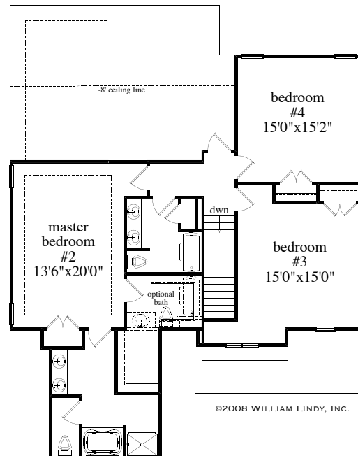
Second Floor: 1062 Sq.Ft.
